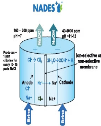
Multiple Chamber Electrolytic Cell
