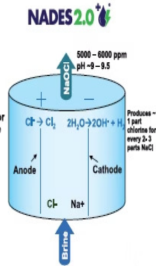
One Chamber Electrolytic Cell
